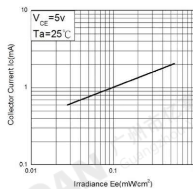
Fig.2 Collector Current vs. Irradiance
