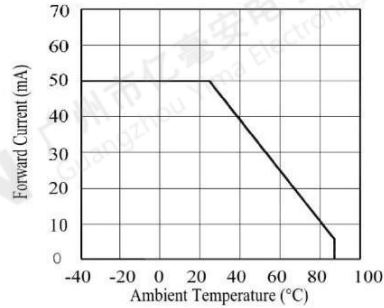
Fig.1 Forward Current vs. Ambient Temperature
