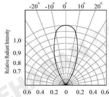
Fig.4 Relative Radiant Intensity vs. Angular Displacement
