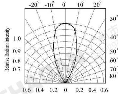
Fig. 4 Relative Radiant Intensity vs. Angular Displacement
