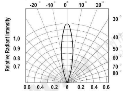
Fig.4 Relative Radiant Intensity vs. Angular Displacement
