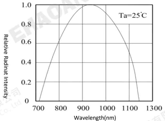
Spectral Sensitivity
