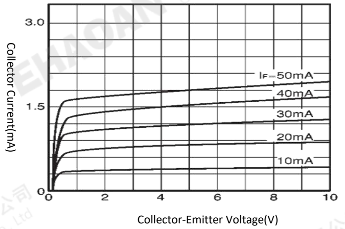
Output Characteristics
