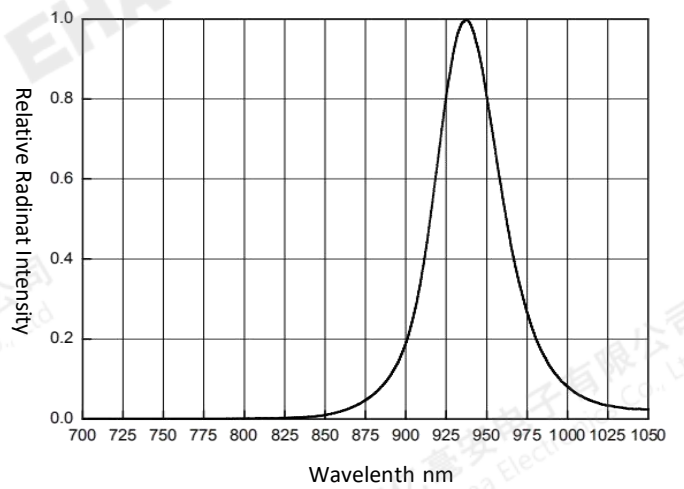
Spectral Distribution
